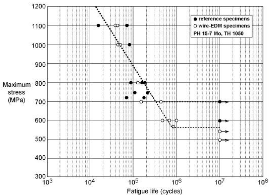
Fig. 5 Effect of wire-EDM on fatigue of PH 15-7 Mo stainless steel (reference specimens were abrasive jet machined, K_t = 1.06 , R = 0.1 ; see subsection 1.5.2)
