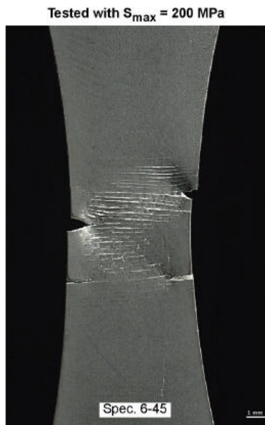
Fig. 7b Example of multiple fatigue crack initiation in a DLC coated specimen [Ref. 8]
