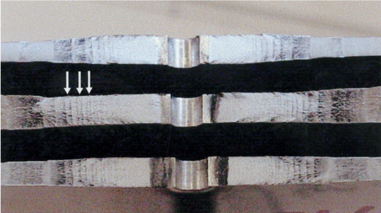
Fig. 8 Fracture surfaces of the three specimens tested with the miniFalstaff load history and S_{\max} = 247.5 , 220 and 230 MPa respectively (top to bottom). The arrows indicate pairs of growth bands associated with the two flights in which the most severe loads are applied (see subsection 1.5.5)
