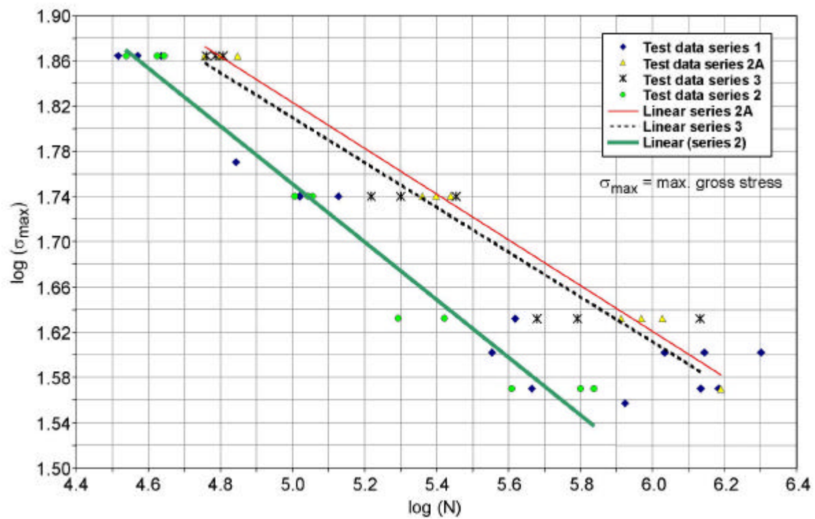
Fig. 3 Fatigue test results for riveted lap joints (subsection 1.5.1a)
