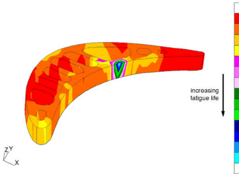
Fig. 2 Calculated fatigue life distribution (cycles) in a single crystal turbine blade (cross-section at half span; see subsection 1.4.2)
