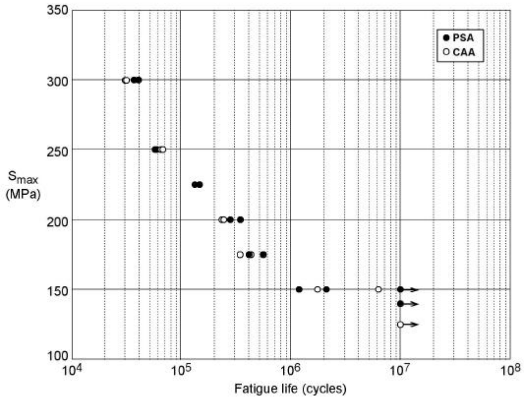
Fig. 6 Comparison of PSA anodised and chromic acid anodised 7075-T6 clad fatigue specimens, K_t = 1.06 , R = 0.1 : (see subsection 1.5.3)
