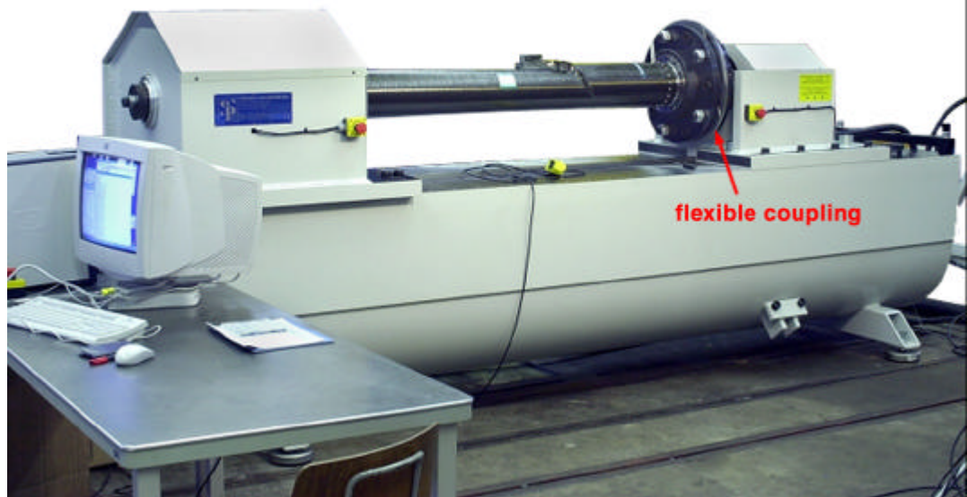
Fig. 10 Torsional fatigue testing of filament wound carbon/epoxy – metal flange drive shafts (see subsection 1.6.1)
