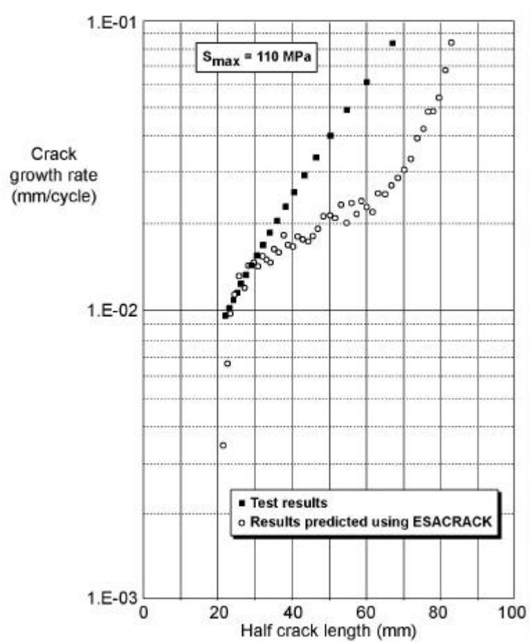
b) Fatigue crack growth rates in FSW panel
