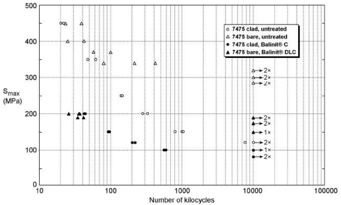
Fig. 7a Fatigue test results for 7475-T761 clad and bare sheet, with and without Diamond-Like-Carbon (DLC) coatings (see subsection 1.5.4)
