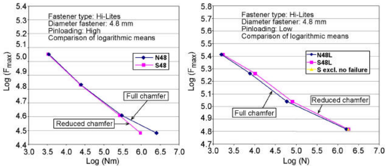
Fig. 4 Example fatigue test results for high and low pin loaded joints (subsection 1.5.1b)
