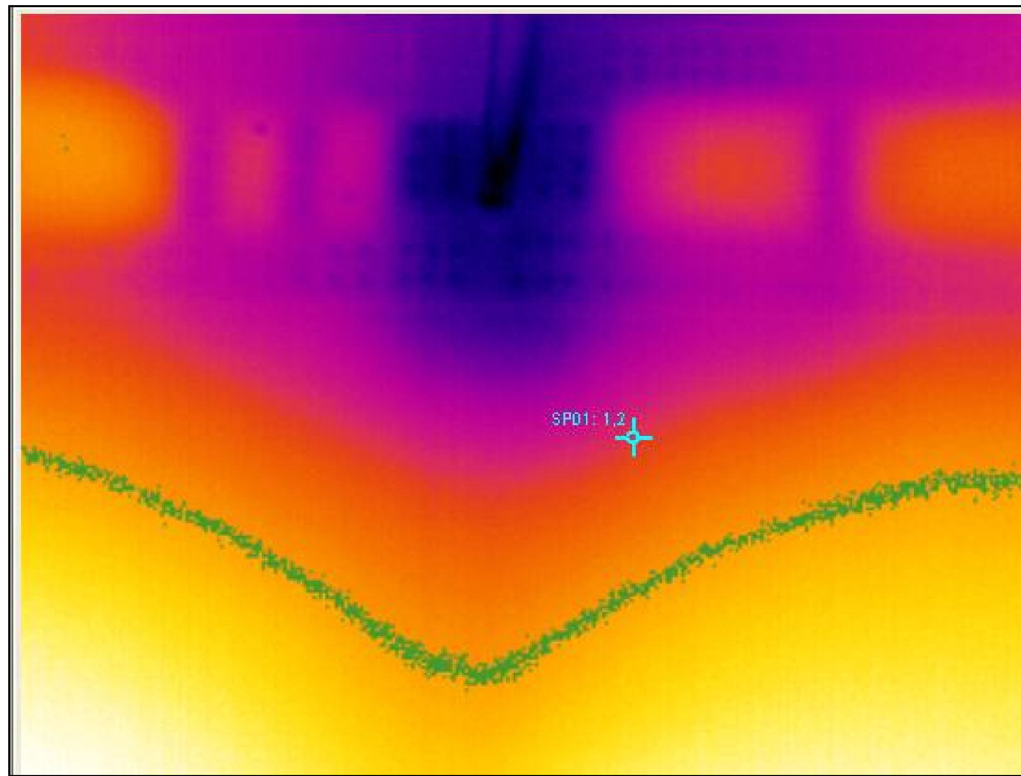
Figure 17: Thermographic inspection of F-18 trailing edge flap (middle hinge) at optimal inspection time (non-defected structure). Picture by courtesy of VTT.
