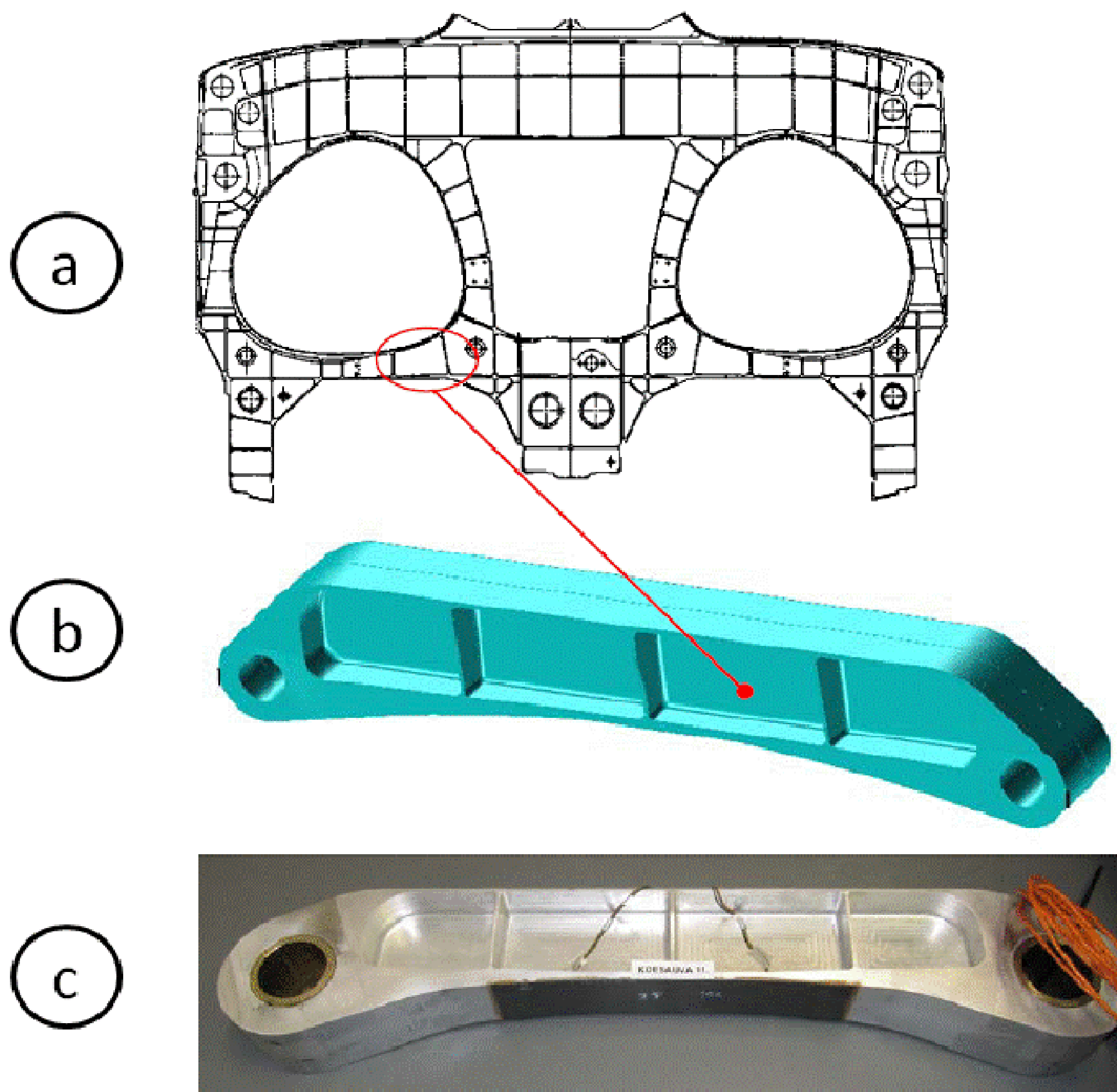
Figure 24: a) The fuselage bulkhead Y488 of the F-18 / 77/; b) model of the specimen emulating the bulkhead; c) actual specimen (№ 11) with the composite patch. Picture by courtesy of Patria Aviation / VTT.
